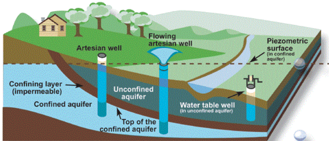
Figure 1: Types of aquifers (USGS 2011)
